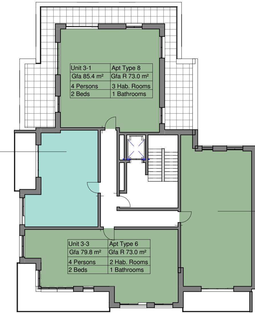
2 L03 FLOOR PLANS Copy 2 1 : 200 @A1
