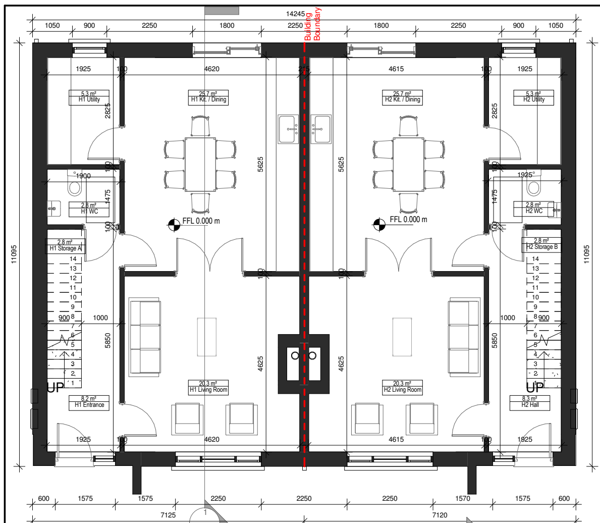
1 00 Ground Floor Plan 1 : 100 @ A3
