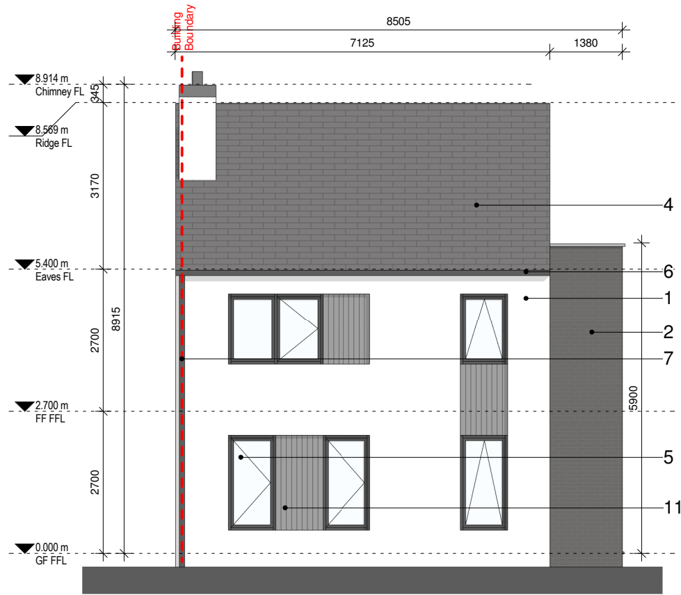
5 01 Front Elevation 1 : 100 @ A3
