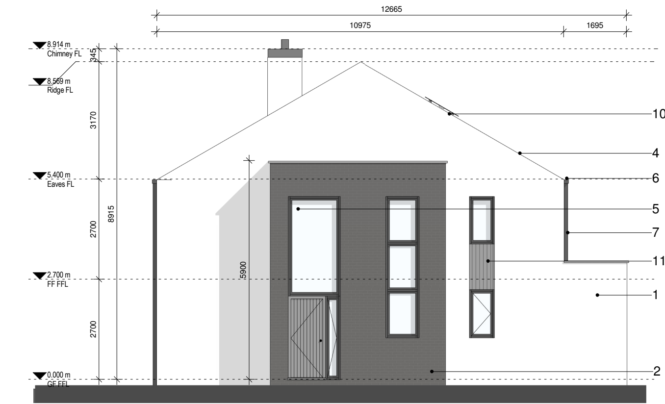
1 04 Side elevation 1 : 100 @ A3
