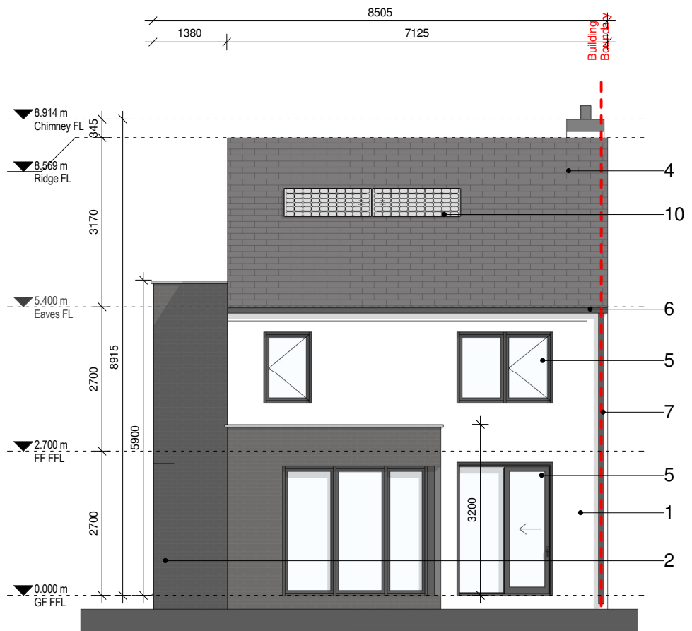
4 03 Rear Elevation 1 : 100 @ A3
