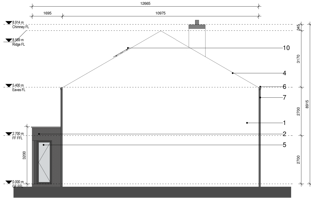
2 02 Side Elevation 1 : 100 @ A3
