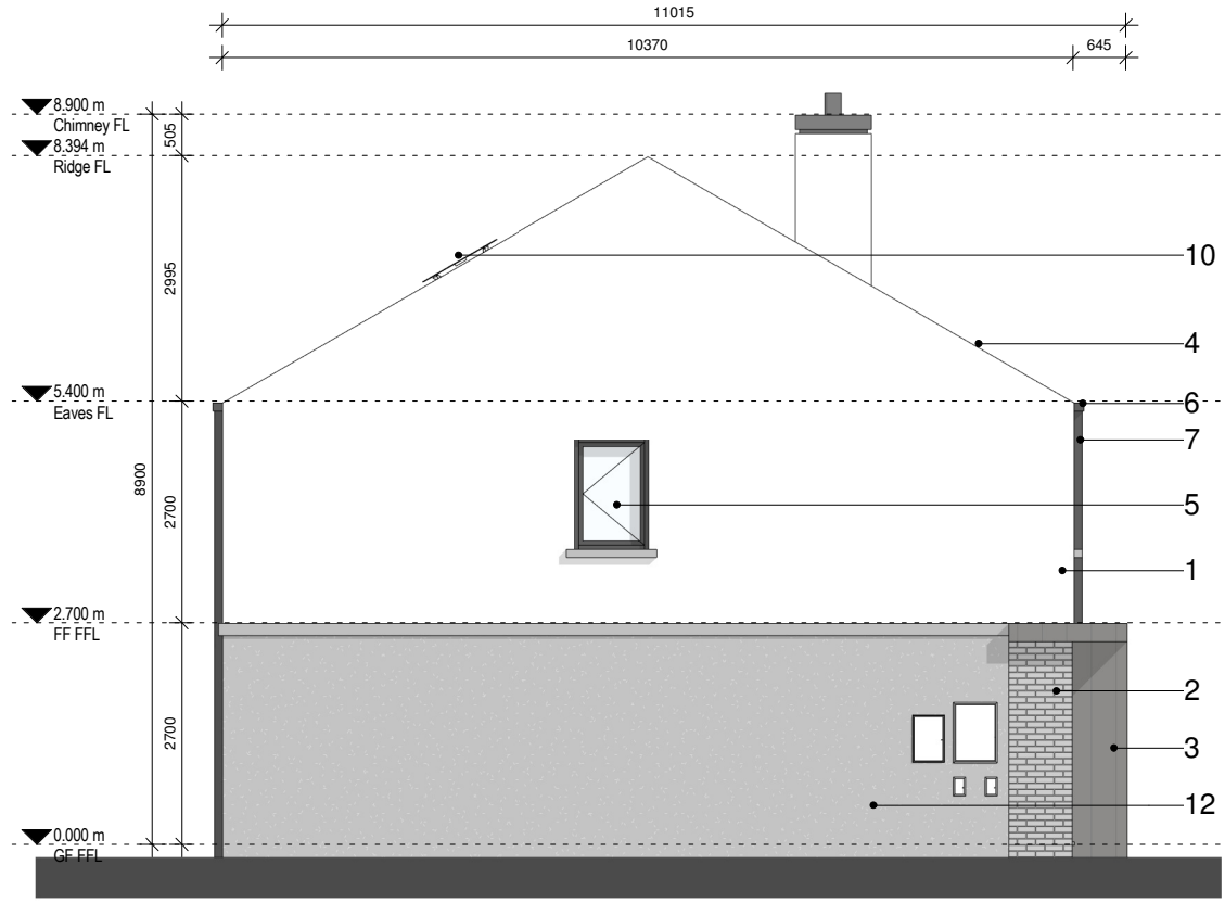
2 02 Side Elevation 1 : 100 @ A3
