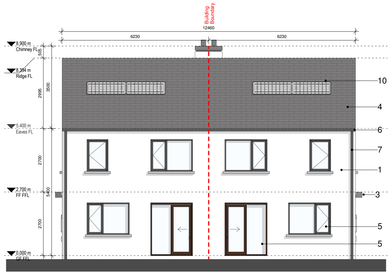
3 03 Rear Elevation 1 : 100 @ A3
