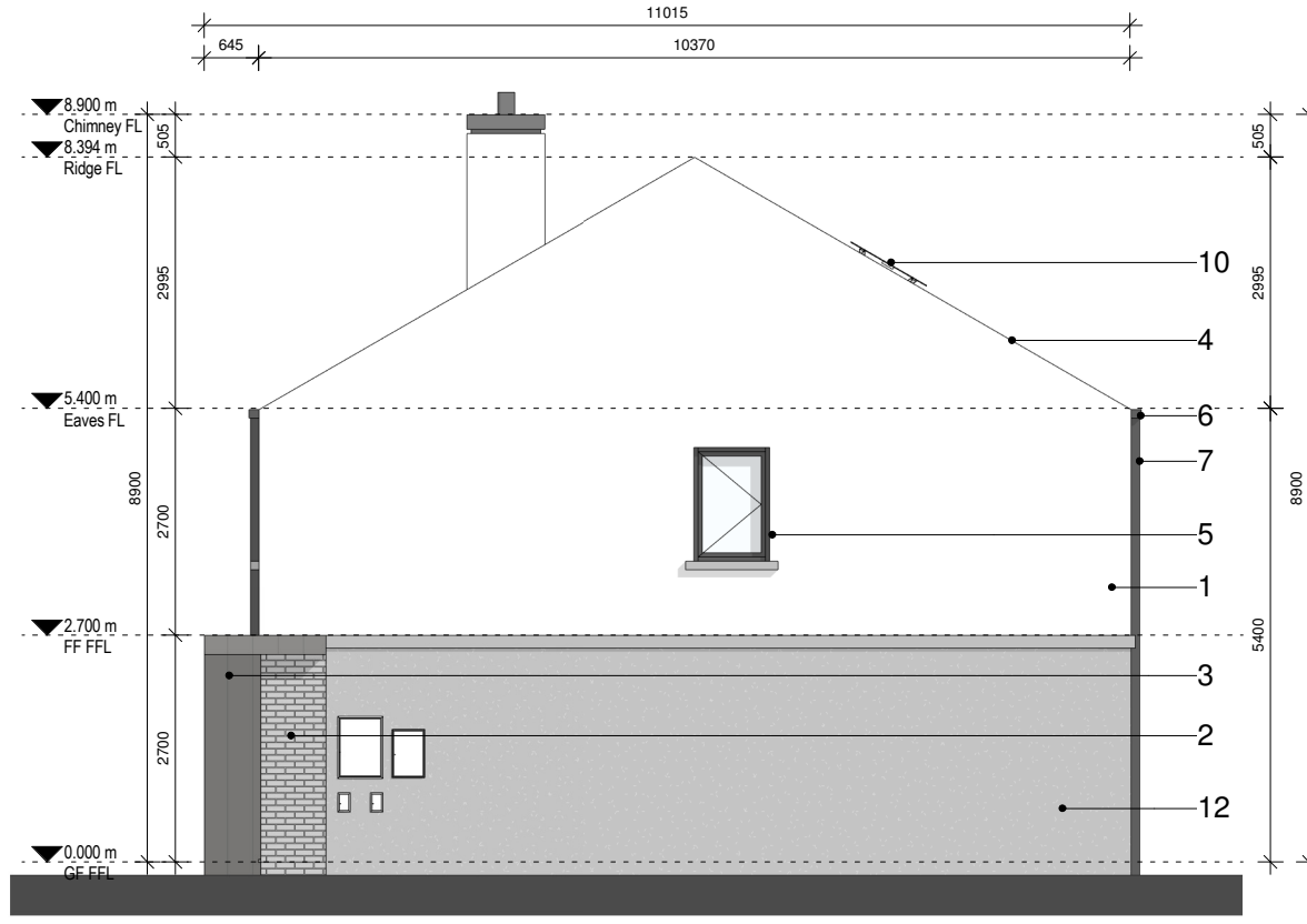
4 04 Side elevation 1 : 100 @ A3
