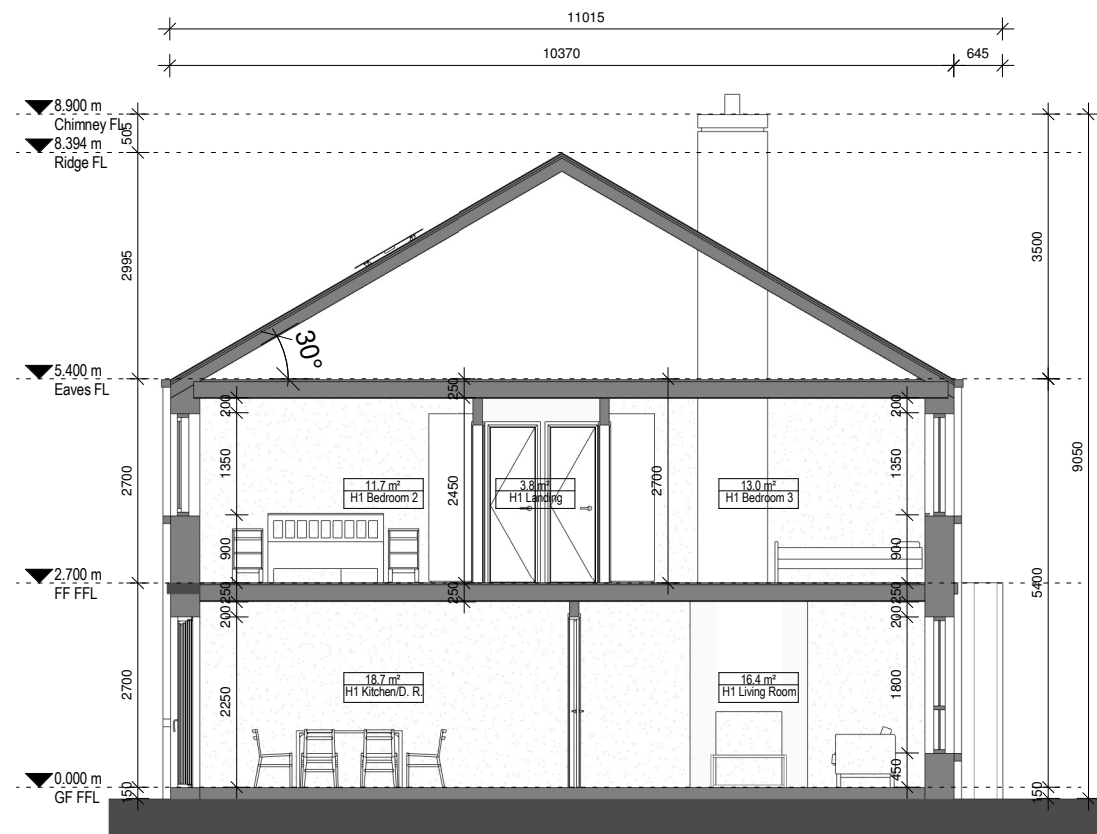
1 Section 1 1 : 100 @ A3
