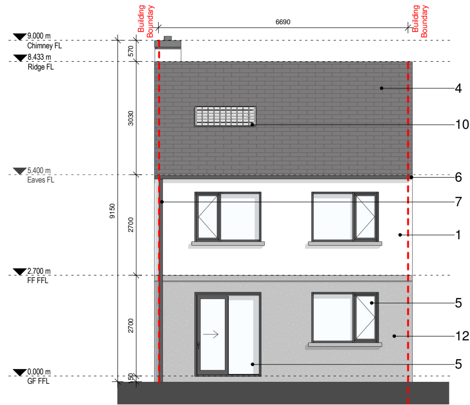
2 Rear Elevation 1 : 100 @ A3
