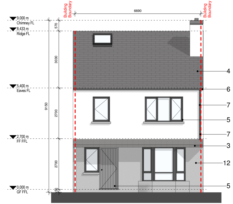
1 Front Elevation 1 : 100 @ A3
