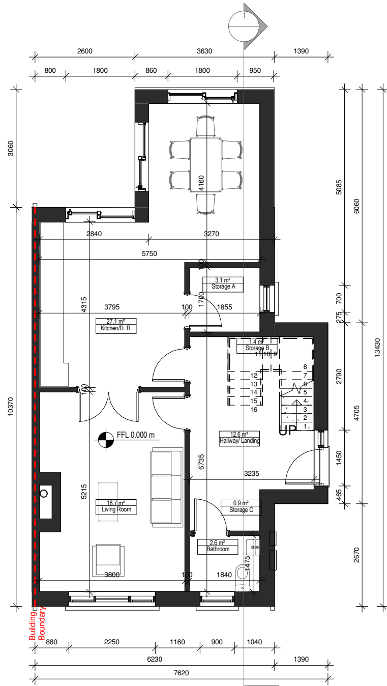
1 00 Ground Floor Plan 1 : 100 @ A3
