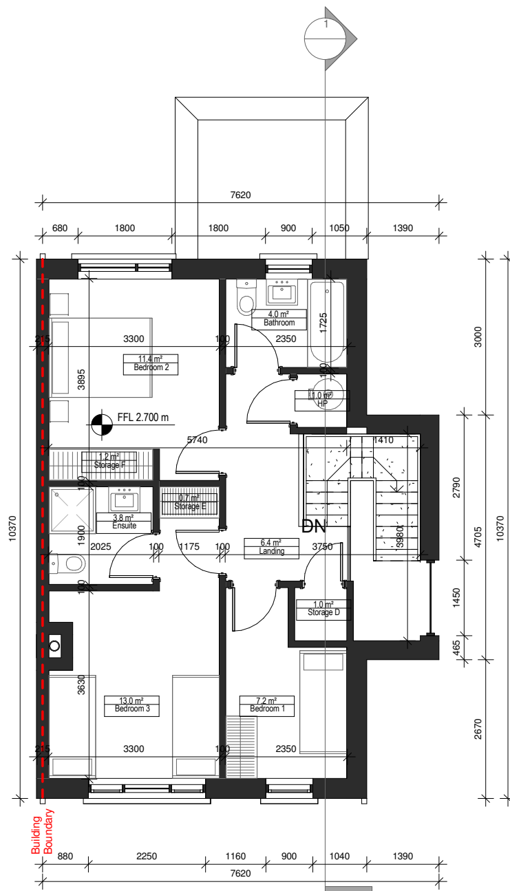
2 01 First Floor Plan 1 : 100 @ A3
