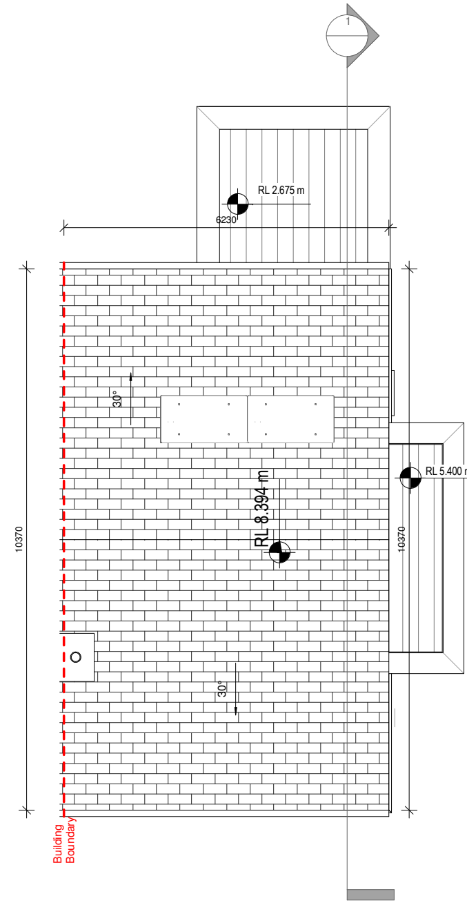
3 03 Roof Plan 1 : 100 @ A3
