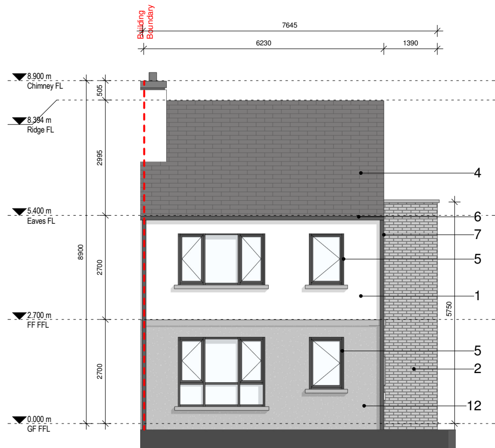
1 01 Front Elevation 1:100 @ A3
