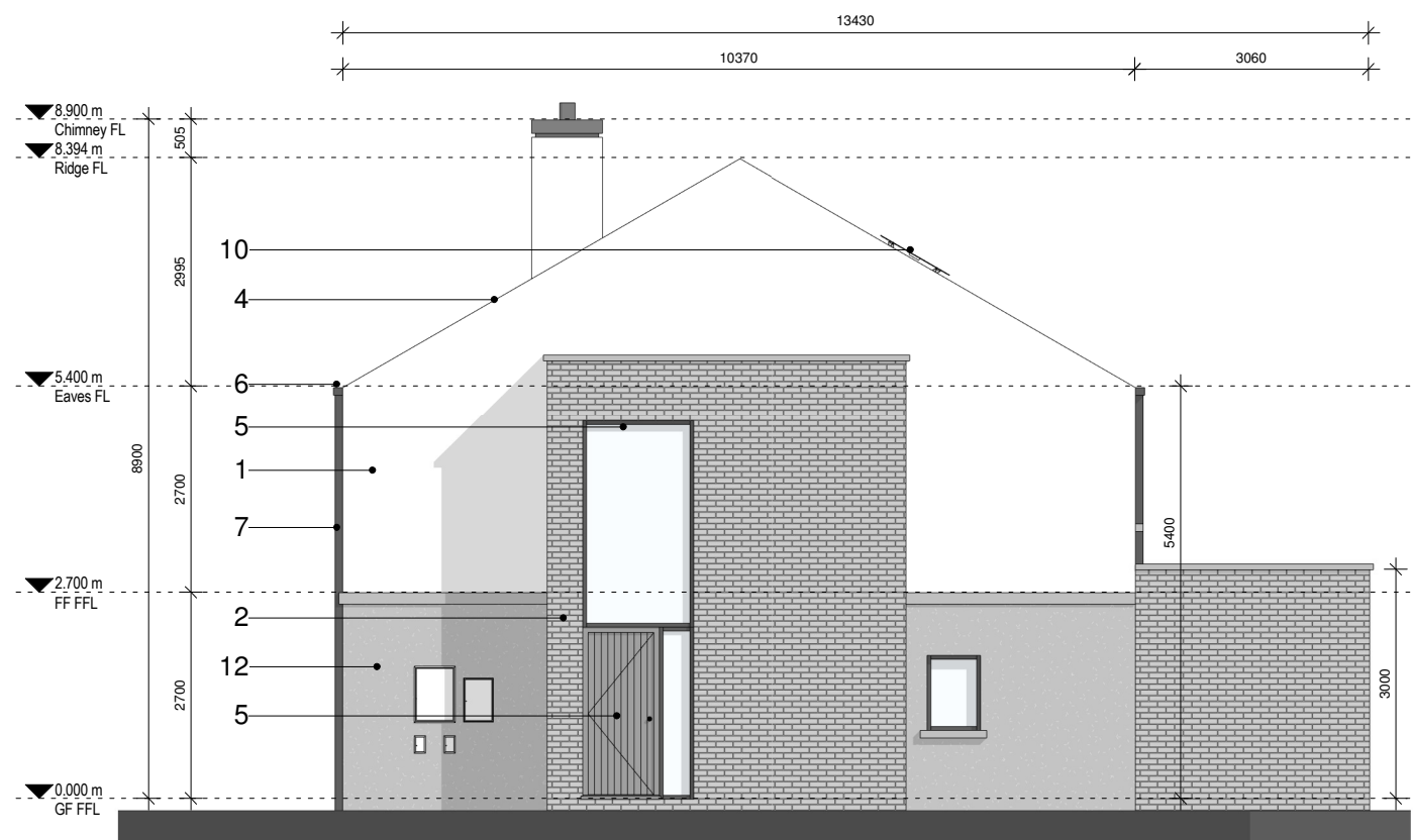
4 04 Side Elevation 1:100 @ A3
