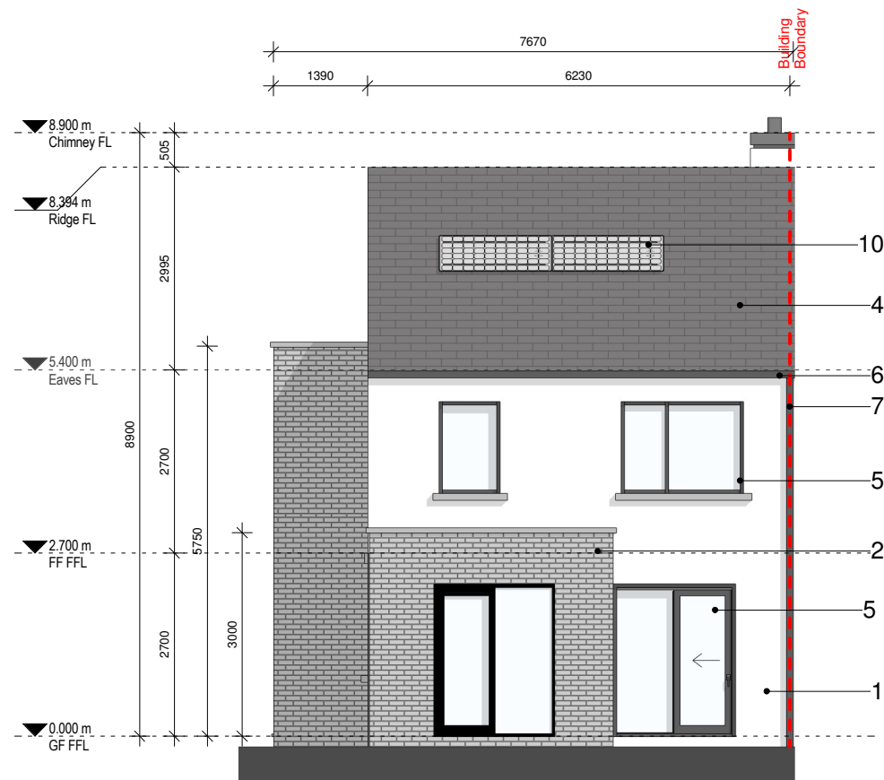
3 03 Rear Elevation 1:100 @ A3
