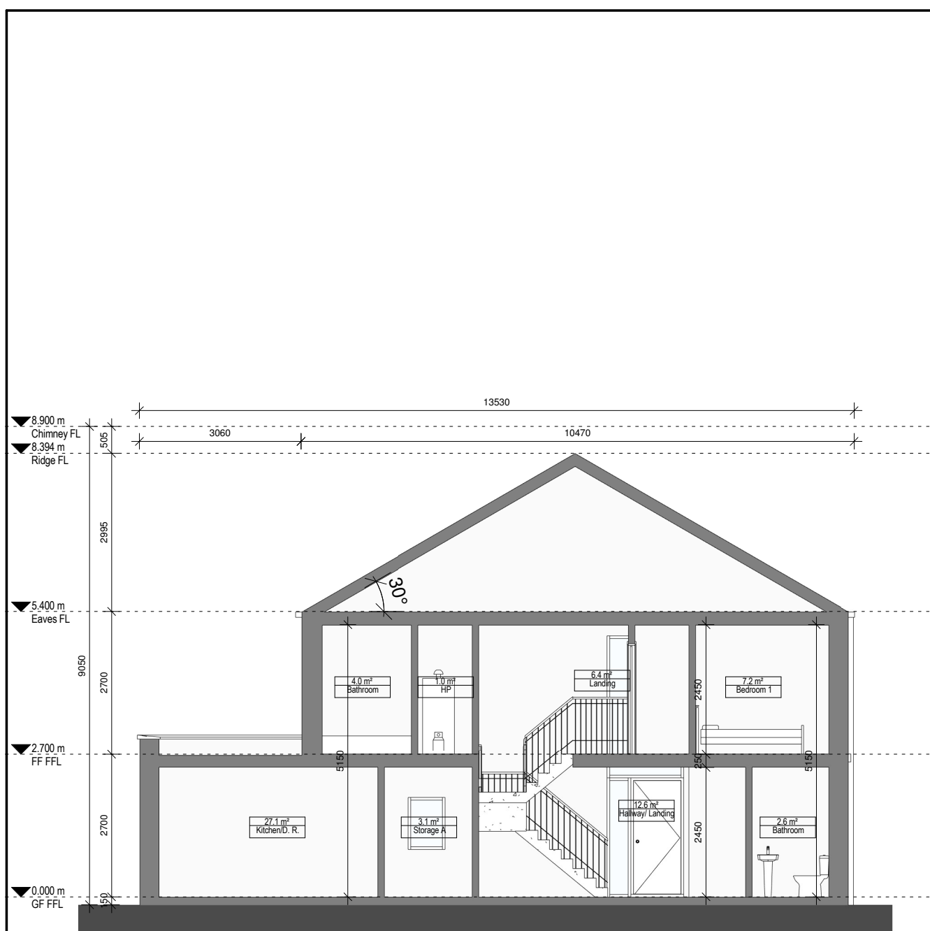
1 Section 1 1 : 100 @ A3
