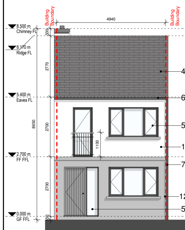
4 Front Elevation 1 : 100 @ A3
