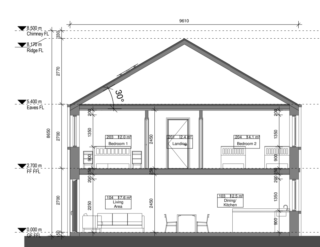
6 Section 1 1 : 100 @ A3
