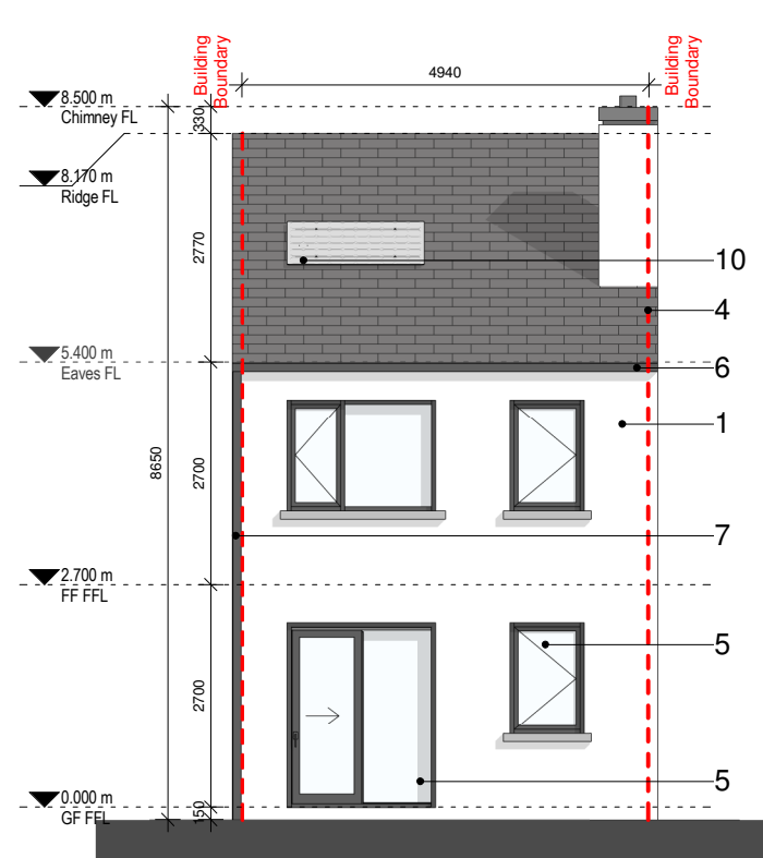
5 Rear Elevation 1 : 100 @ A3
